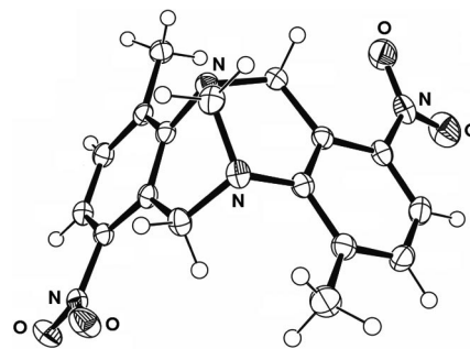
Figure 4. An ORTEP diagram of 15 with 50% probability ellipsoids.
